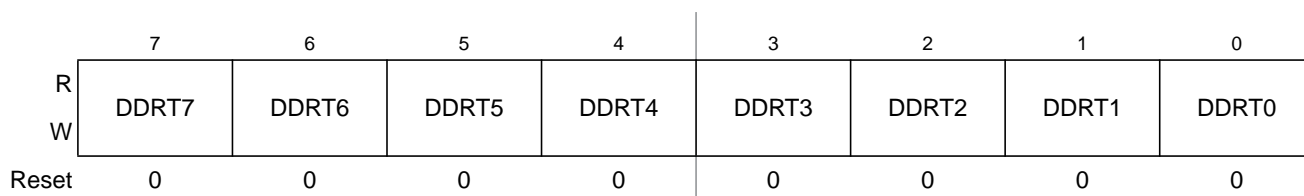
Figure 23-21. Port T Data Direction Register (DDRT)
